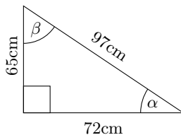
Figure 5.5: A right triangle
