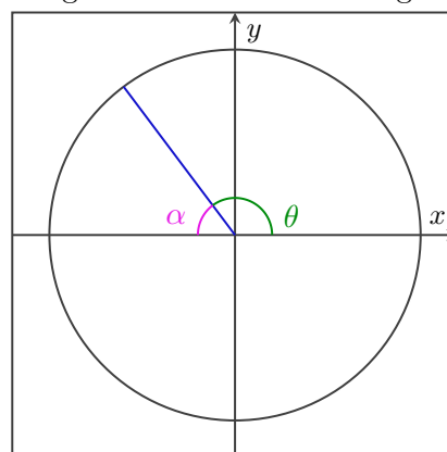
Figure 5.11: Reference Angles
