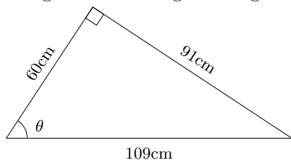
Figure 5.14: A right triangle
