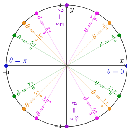
Figure 5.2: Standard Angles
