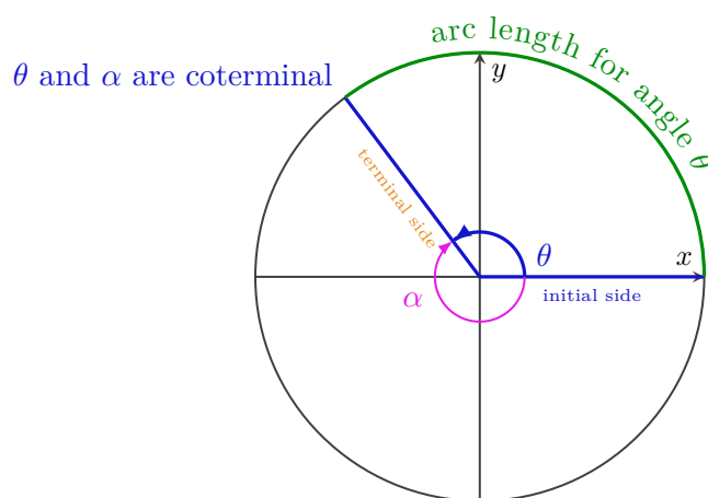
Figure 5.3: Coterminal angles \theta and \alpha
