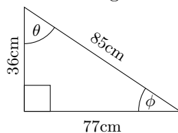
Figure 5.8: A right triangle
