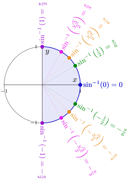
Figure 6.16: Unit Circle with Standard Inverse Sine Values
