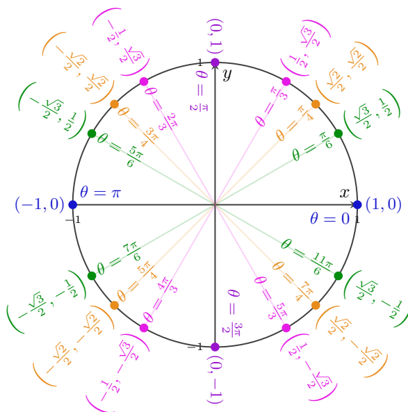
Figure 5.12: Unit Circle with Standard Values
