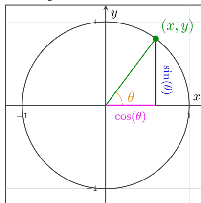
Figure 5.10: Unit Circle
