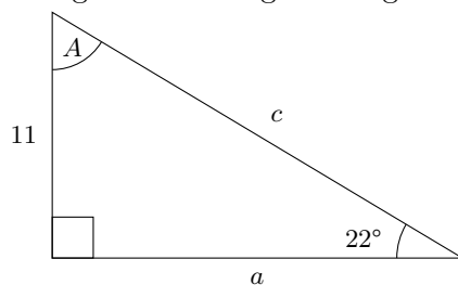
Figure 5.9: A right triangle
