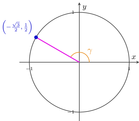
Figure 5.13: A point on a unit circle at an angle \gamma
