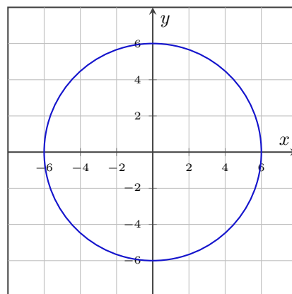
Figure 5.4: A circle of radius 6
