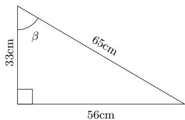
Figure 5.18: A right triangle
