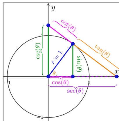
Figure 5.15: Other trigonometric function definitions
